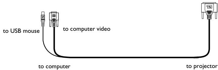
FIGURE 5 MI-DA analog computer cable
